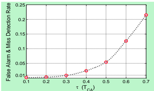
Fig. 2. False alarm rate and missed detection rate as a function of the multipath delay time. The multipath signal power is 10 dB below its direct signal power.
