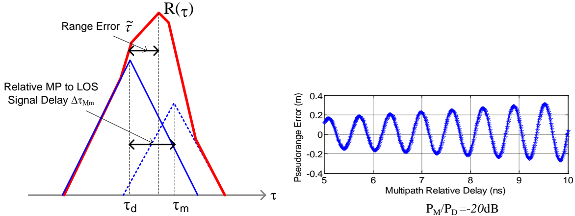
Fig. 1. Schematics of GPS multipath impact on range measurements and simulated pseudorange error for weak multipath with relatively short delay time.
