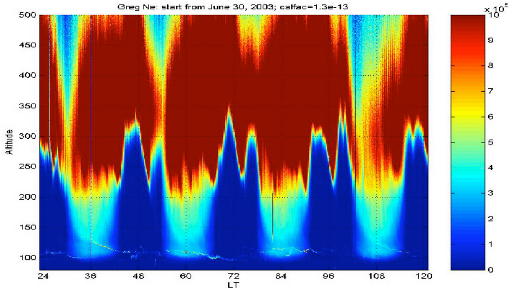
Electron density distributions as a function of local observation time and altitude obtained using the incoherent scatter radar in Arecibo, Puerto Rico.
